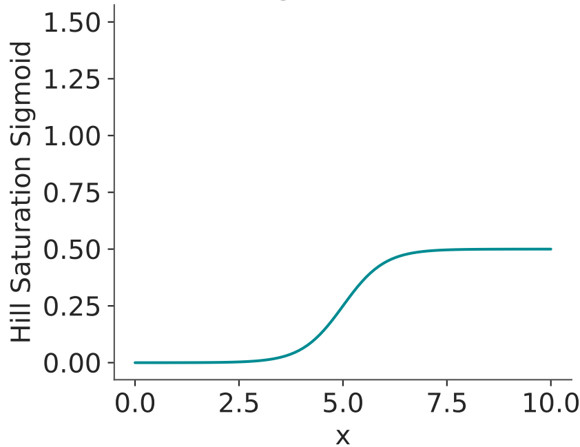
Sigma = 0.5
