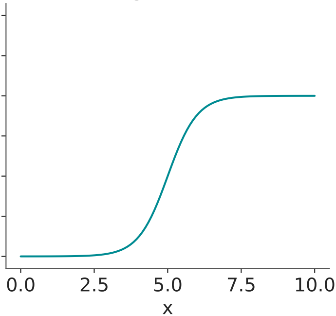
Sigma = 1
