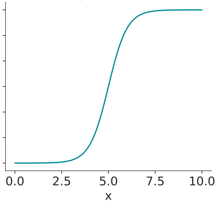
Sigma = 1.5
